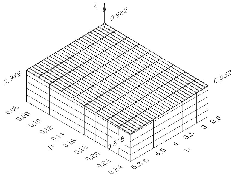
Figure 6: Values of k as a function of friction coefficient \mu and the instantaneous h height of the piece ( H_0 = 5.3\text{mm} , R_0 = 8\text{mm} , k = 1.23602 - 0.977926\mu - 0.0865165h )
